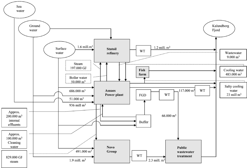
Figure 2 Selected industrial symbiosis water flows in Kalundborg ( \text{m}^3/\text{yr} and \text{GJ}/\text{yr} ) in 2002. Source: Green Accounts from Statoil, 2002, Novo Group, 2002, and Asnæs power plant, 2002 and information from the companies obtained through the Kalundborg Center for Industrial Symbiosis (Hansen 2004). WT = wastewater treatment; FGD = fluegas desulfurization; mill. = million. One gigajoule (GJ) = 10^9 joules (J, SI) \approx 2.39 \times 10^5 kilocalories (kcal) \approx 9.48 \times 10^5 British thermal units (BTU); one cubic meter ( \text{m}^3 , SI) = 10^3 liters (L) \approx 264.2 gallons (gal).
